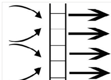
Integrated flow straightener - no inlet section necessary
